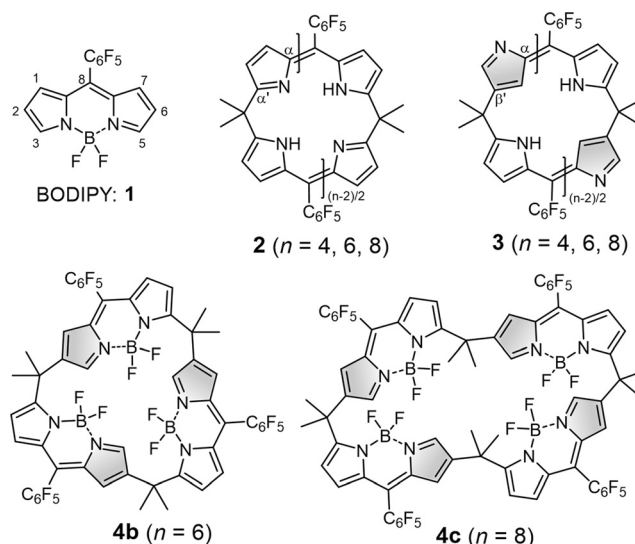
Scheme 1. Chemical structures of meso -C 6 F 5 -BODIPY ( 1 ), calix[ n ]phyrin ( 2 : n = 4, 6, 8), N-confused calix[ n ]phyrin ( 3 : n = 4, 6, 8), and their boron difluoride complexes ( 4b : n = 6; 4c : n = 8).
